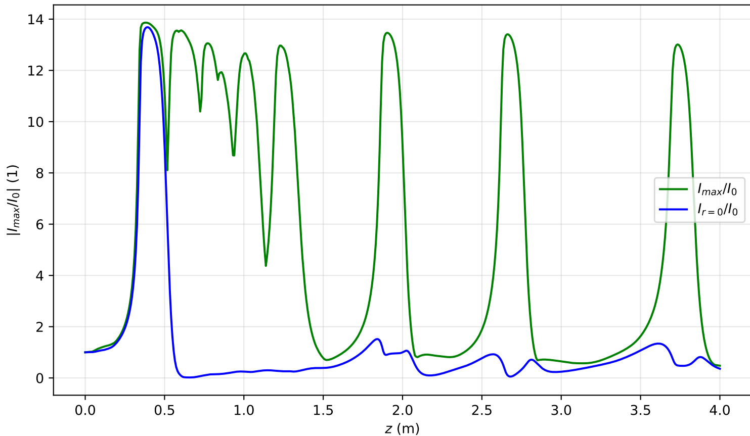
I_{max}(x=0, y=0, z)/I_0 , Pin=8.0Pcr, noisy input, artificial time
